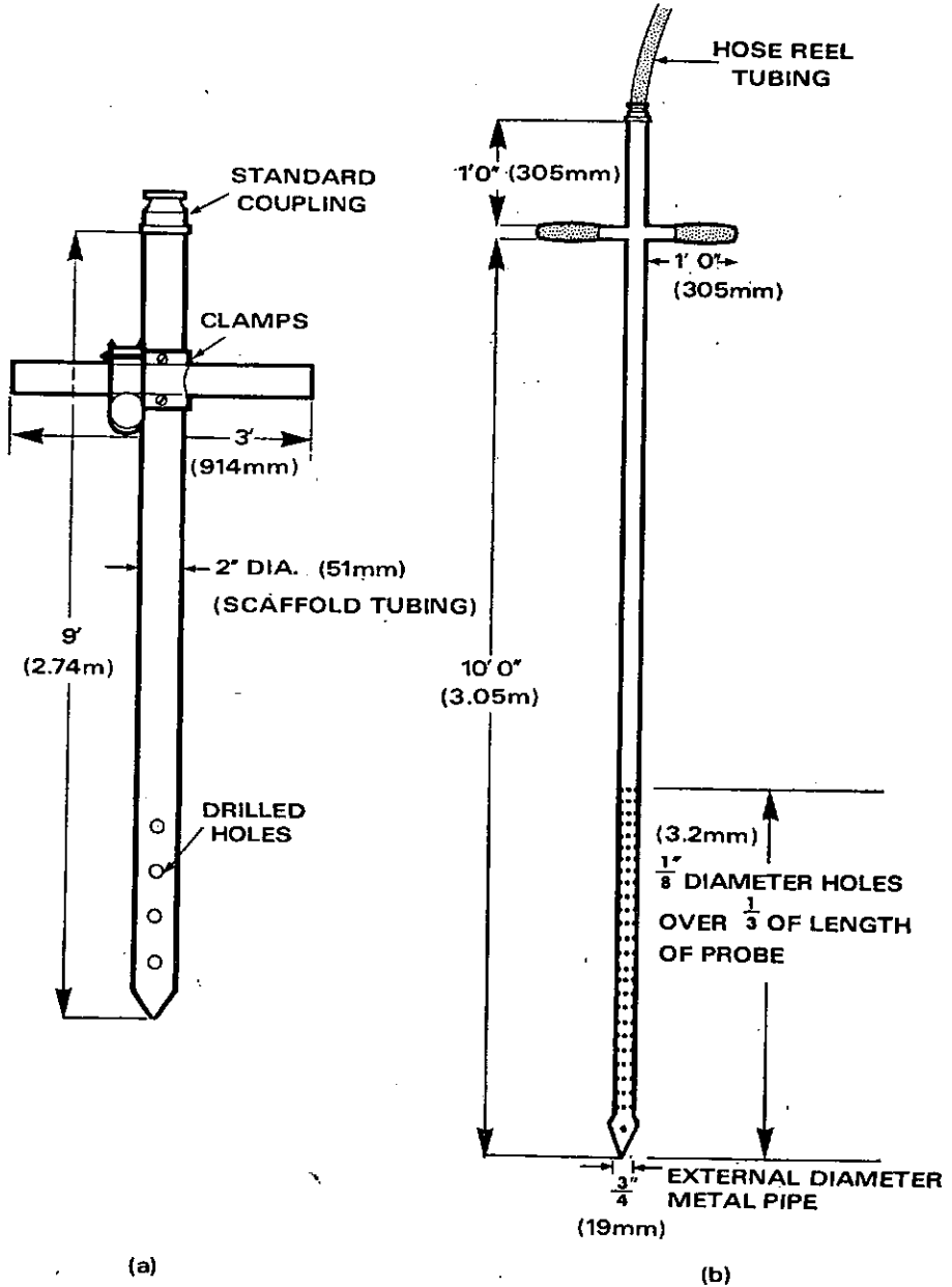
EXAMPLES OF WATER PROBE
